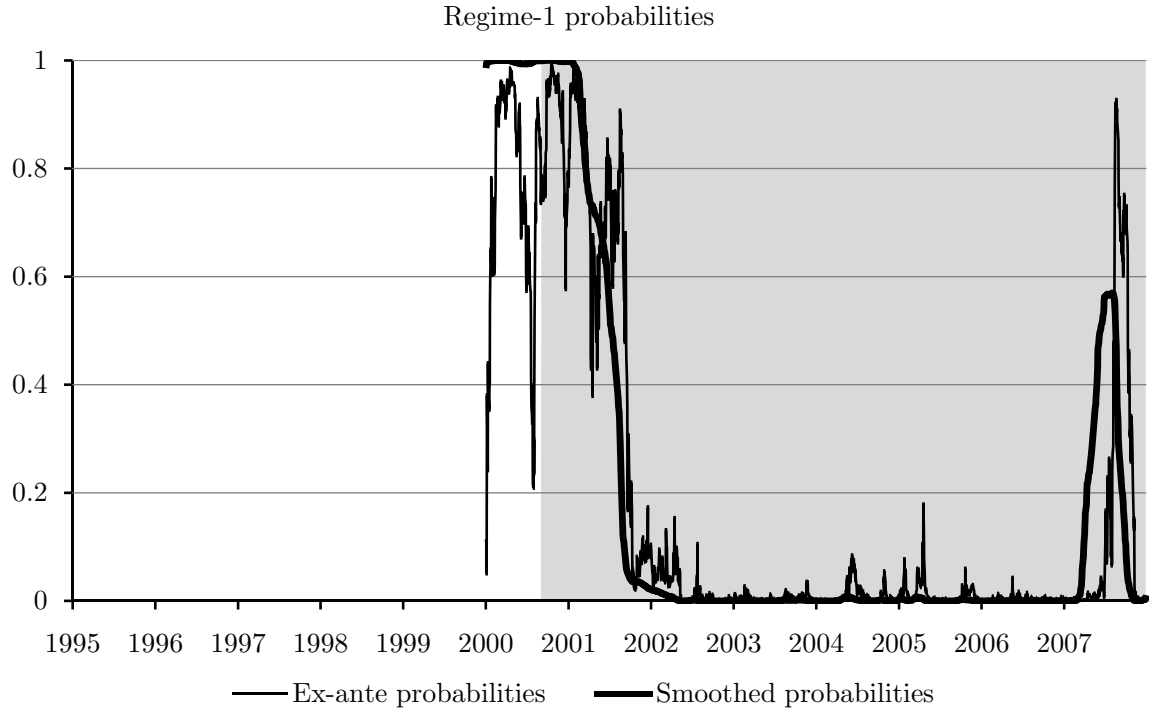
Figure 4: Regime-1 probabilities and conditional variances (TechWIG)
