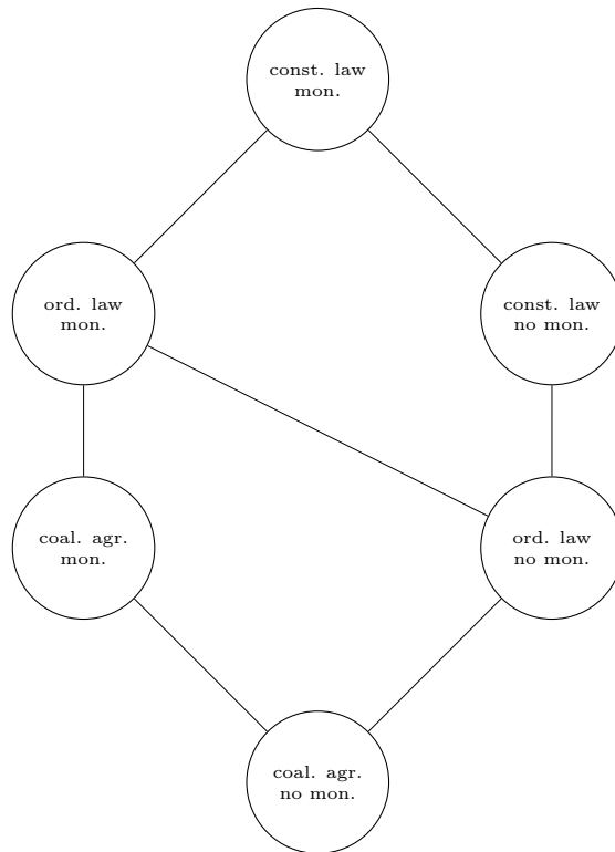
Figure 1: Hasse diagram
